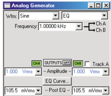
Figure 55. Analog Generator Sine EQ
