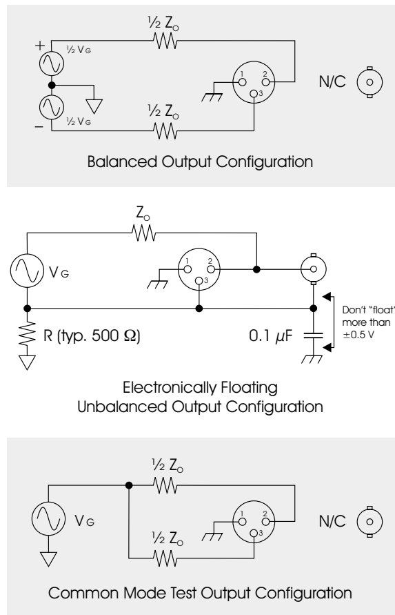
Figure 10. Analog Output Circuit Configurations, simplified.
