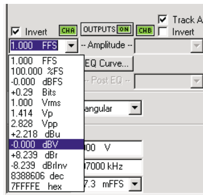
Figure 73. Setting the Digital Generator Amplitude.
