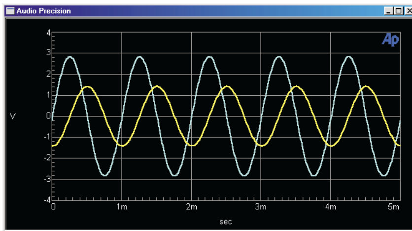
Figure 79. Sine: Var Phase , triggered on Channel A (the larger waveform). -90.00 deg has been entered in Phase B–A field, causing B (the smaller waveform) to lag A.
