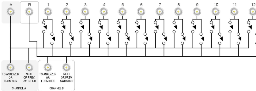
Figure 295. Unbalanced Switcher simplified schematic.
