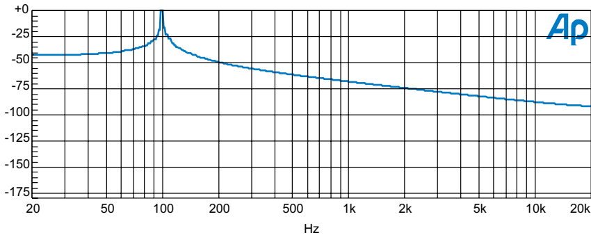
Figure 319. Non-synchronous FFT with no windowing function, 100 Hz sine wave.
