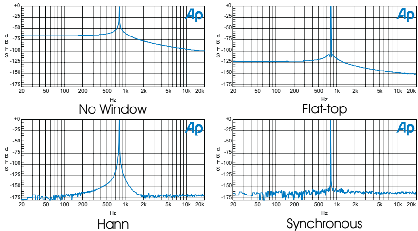
Figure 322. FFTs of 800 Hz sinewave, with no window, Flat Top window, Hann window, and, finally, adjusted very slightly in frequency (to 799.805 Hz) to be synchronous.
