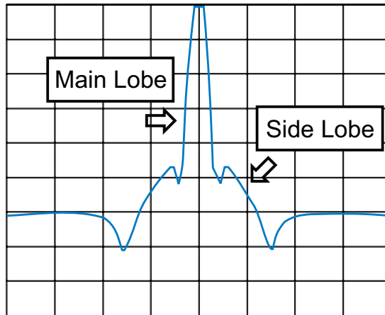
Figure 321. Example of a Blackman-Harris window function viewed in the frequency domain.
