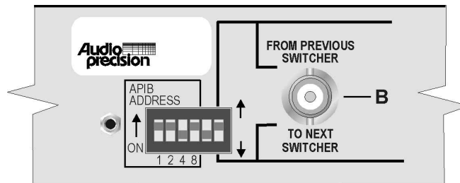
Figure 303. Unbalanced switcher rear panel APIB DIP switch with address/mode switching.
