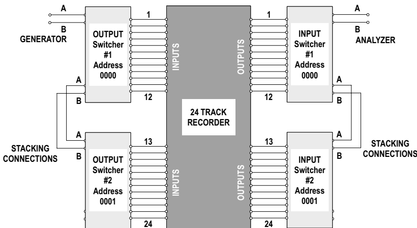
Figure 286. Switcher signal connection and address configuration diagram for a typical multitrack recorder test setup.
