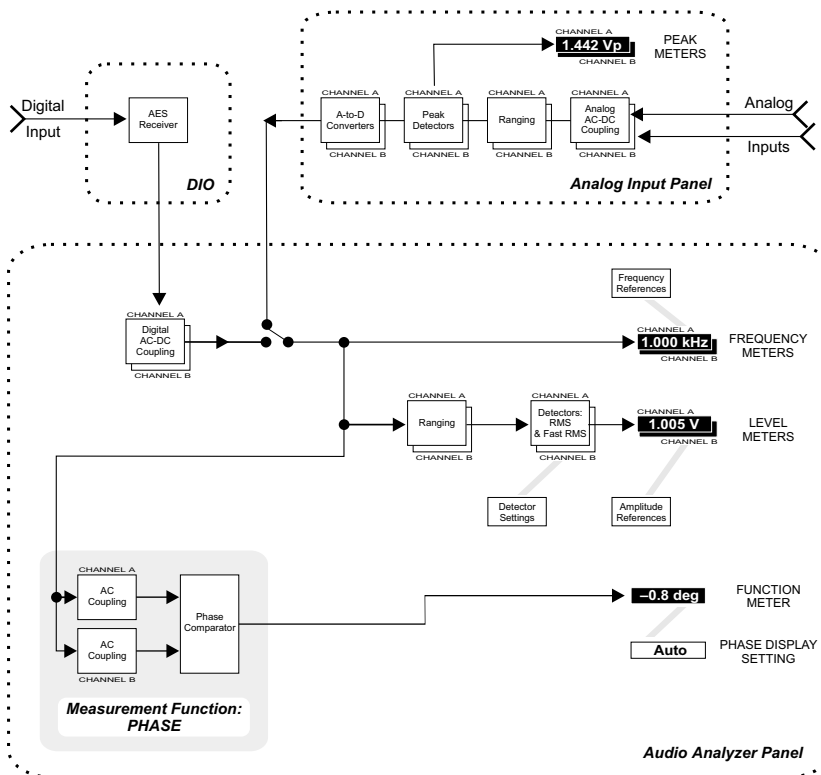
Figure 115. Conceptual Block Diagram, Phase Function.
