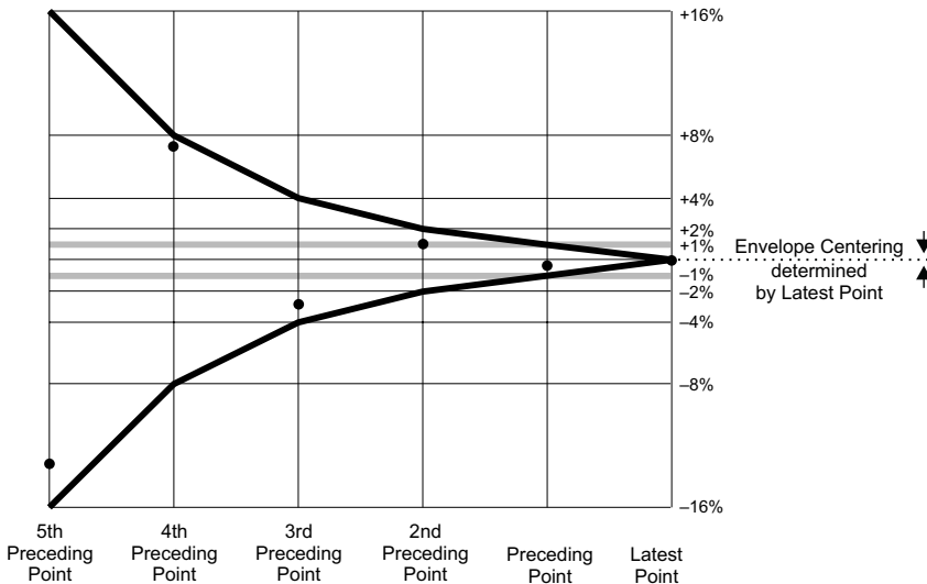
Figure 221. Successfully settled reading using Exponential method, where Tolerance is set to 1 % and Points is set to 5.
