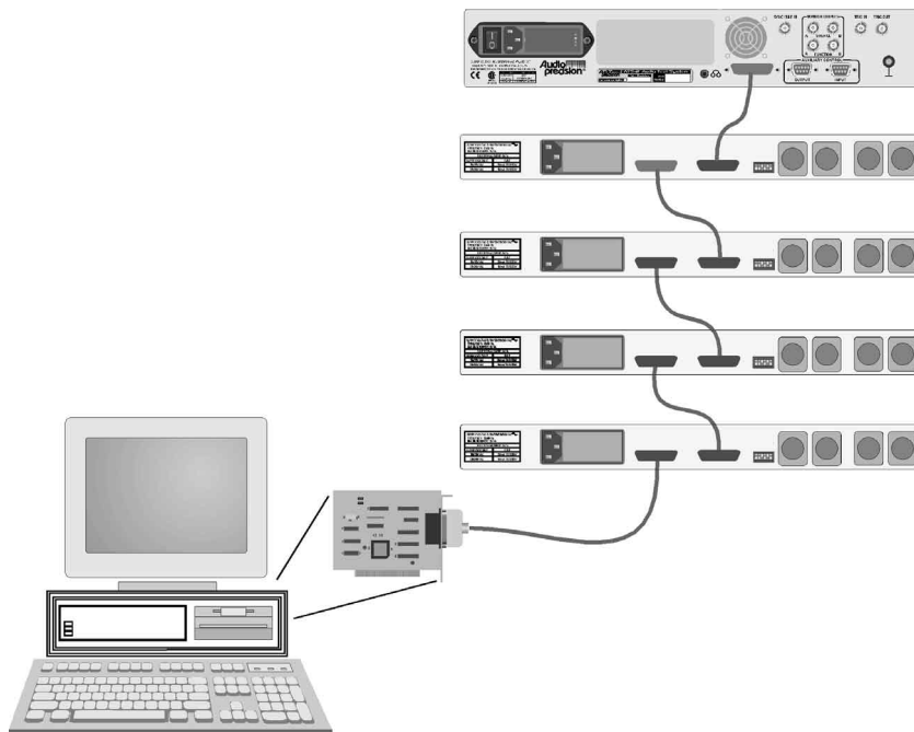
Figure 299. Block diagram, typical APIB "daisy chain" connections.
