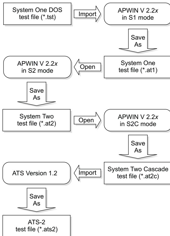
Figure 323. Preparing a test file for translation from S1.EXE or APWIN to an ATS-2 compatible test file.
