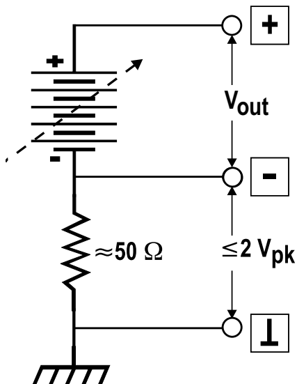
Figure 310. Equivalent circuit, DC OUTPUT 1 or 2
