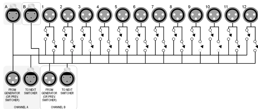
Figure 292. Output Switcher simplified schematic.
