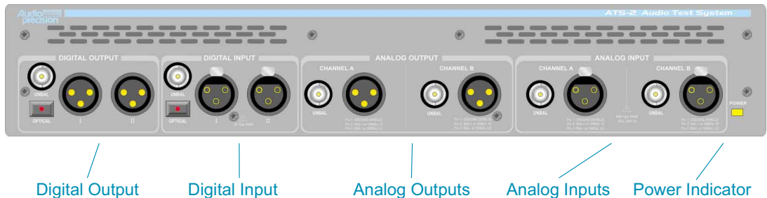
Figure 9. ATS-2 Front Panel
