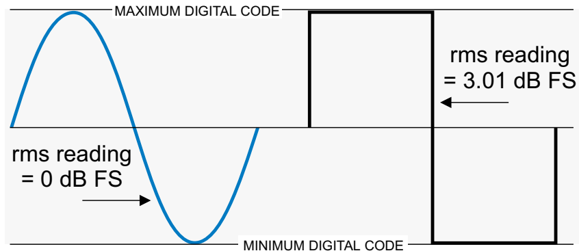
Figure 313. The squarewave has a lower crest factor than the sinewave. Since dBFS is defined in rms terms, a squarewave with the same peak value as a 0 dBFS sinewave will have a value of 3.01 dBFS.
