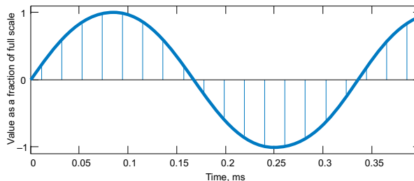
Figure 314. A 3 kHz sinewave sampled at 48 kHz.
