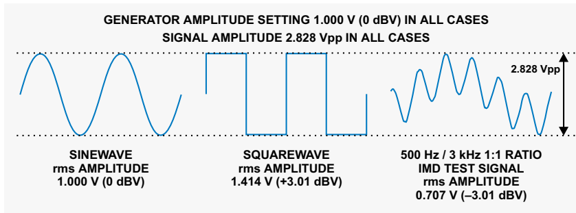
Figure 312. ATS-2 generator output calibrations
