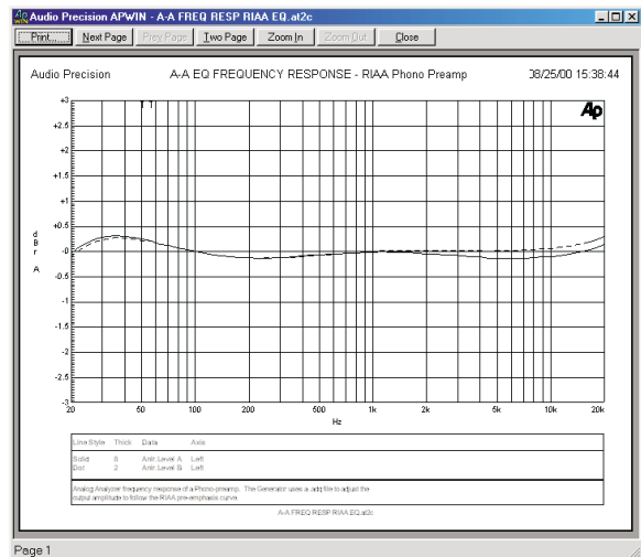
Figure 261. Print Preview.
