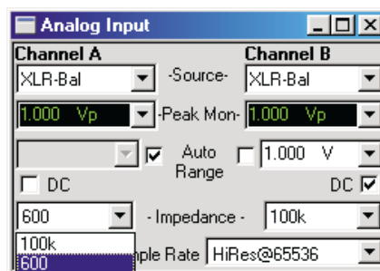
Figure 14. The ATS-2 Analog Input panel, shown with the 600Z impedance option.
