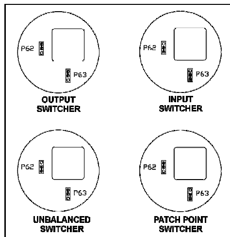
Figure 301. P62 and P63 jumper placement for Output, Input, Patch Point and Unbalanced switchers.
