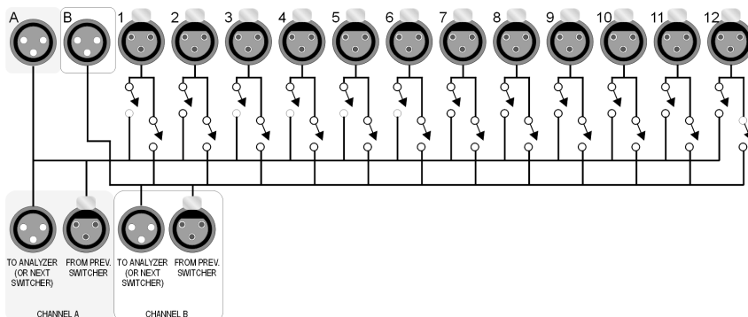
Figure 289. Input Switcher simplified schematic.
