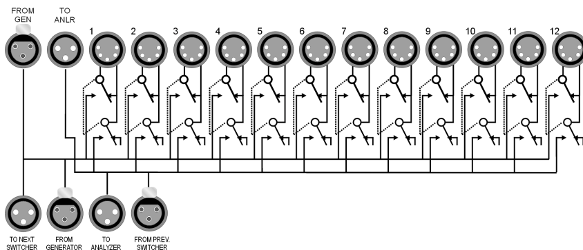
Figure 298. Patch Point Switcher simplified schematic.
