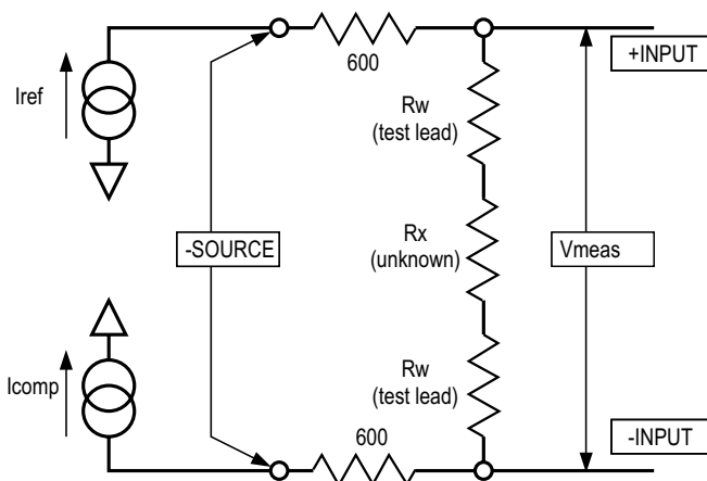
Figure 308. Simplified diagram of 2-wire ohmmeter operation.
