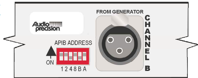
Figure 302. Typical switcher rear panel APIB DIP switch.
