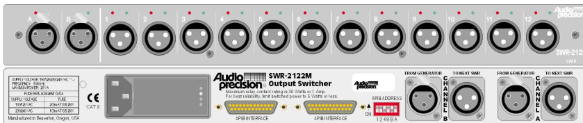
Figure 283. An Audio Precision SWR-2122M Output Switcher, front and rear panels.
