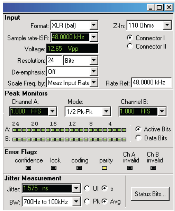
Figure 25. The DIO Input Section.
