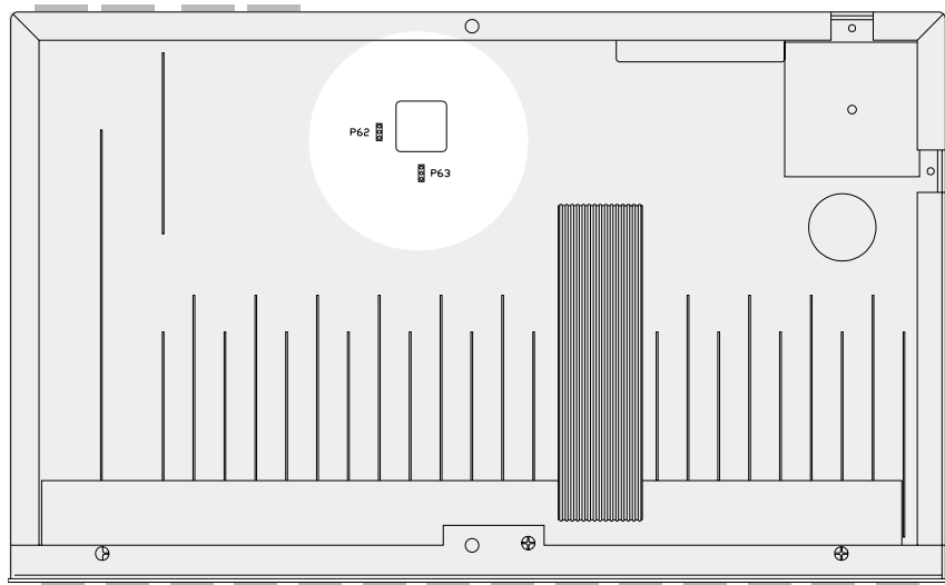
Figure 300. P62 and P63 jumper locations inside SWR-2122 switchers.
