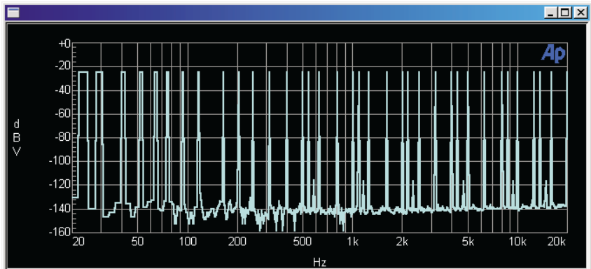
Figure 173. Spectrum View of Typical Multitone Stimulus Signal.
