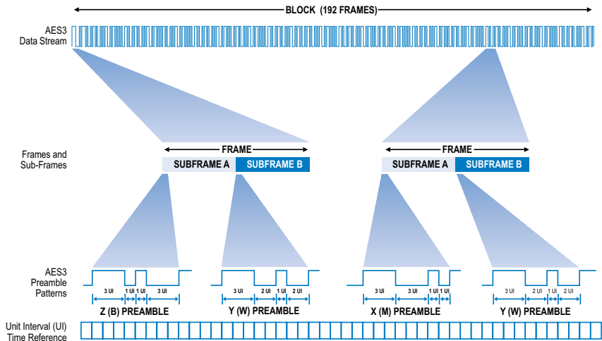
Figure 315. The AES3 serial interface signal data pattern.
