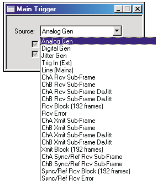
Figure 271. The Main Trigger source list.
