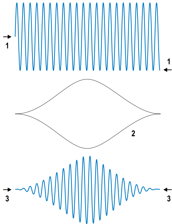
Figure 320. Application of a Hann window function (raised cosine shape) to a sinewave, viewed in the time domain.
