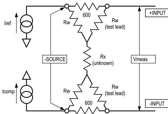
Figure 309. Simplified diagram of 4-wire ohmmeter operation.
