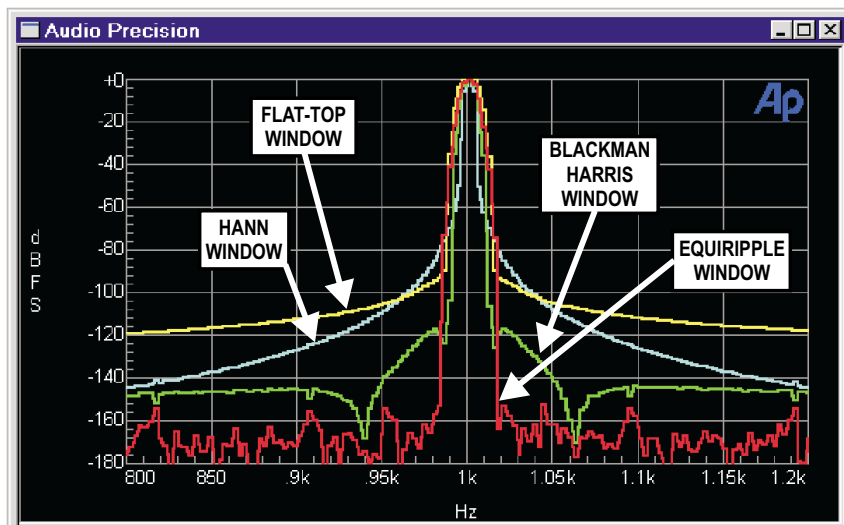
Figure 134. FFT Window Functions: Flat-Top, Hann, Blackman-Harris and Equiripple.
